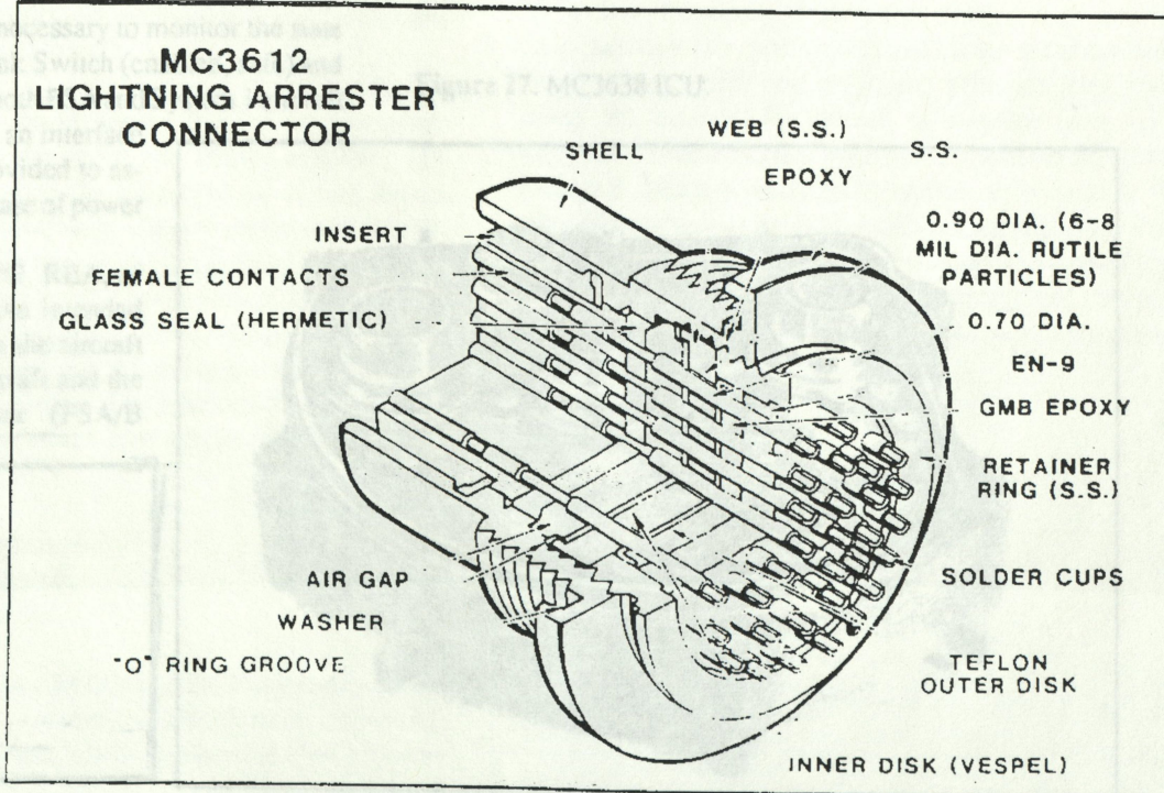
Figure 25. MC3612 Lightning Arrestor Connector
